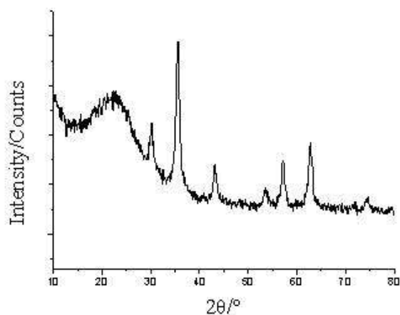
Fig. 2 XRD pattern of MMIPs
